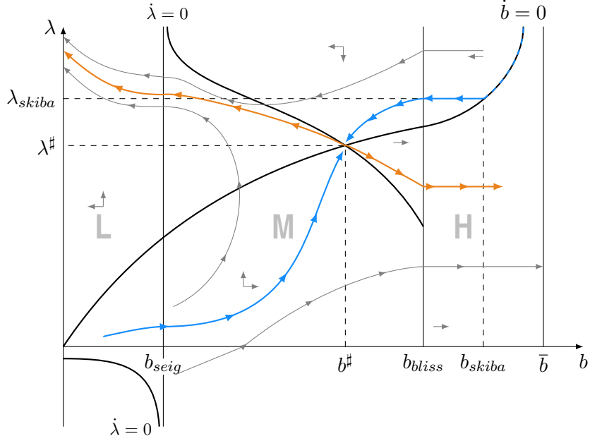
Figure 2: Benchmark, with \psi_{bliss} > \gamma_{bliss} .
