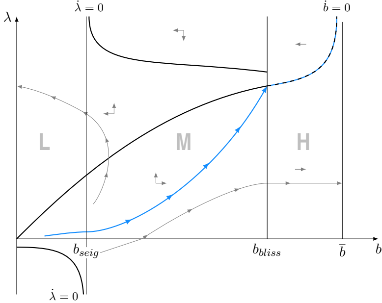
Figure 1: Benchmark, with \psi_{bliss} < \gamma_{bliss} .
