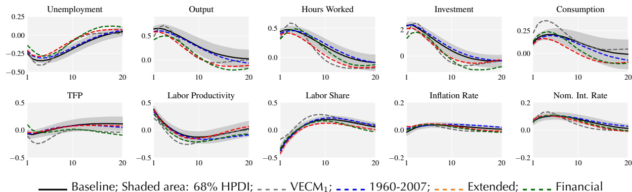
Figure 5: Robustness, IRFs
