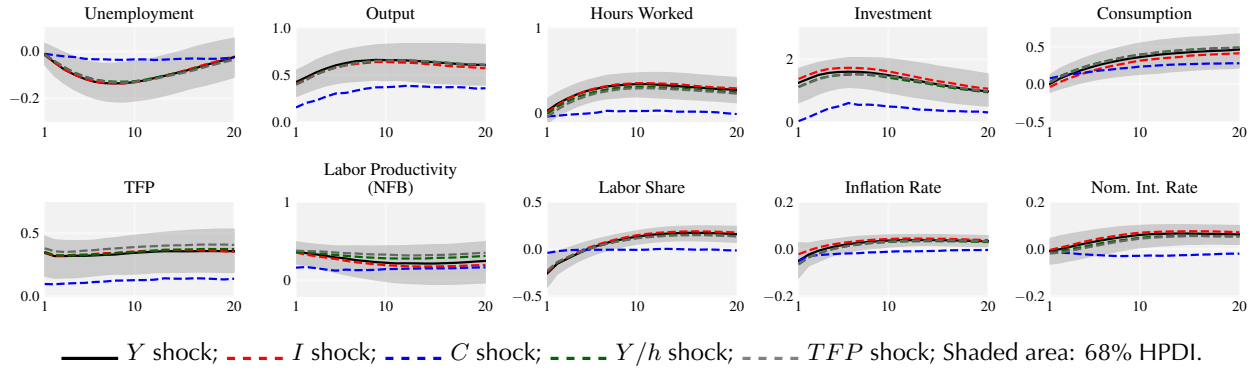
Figure 3: Long-Run Shocks
